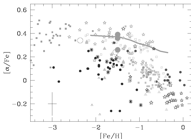
FIG. 12.—[ \alpha /Fe] vs. [Fe/H] for a variety of halo and extragalactic samples (see text for full explanation). Light gray symbols represent halo samples, black are for low-mass dSphs, dark gray for Sgr, light gray for the LMC, and light gray for dIrrs. In detail, solid light gray curve and light gray stars; Gratton et al. (2003) dissipative collapse and accreted halo stars, respectively; small light gray filled circles; NS97 low- \alpha stars; mean values for the three F02 components as the large light gray filled circles; mean points for three different metallicity bins from Stephens & Boesgaard (2002); large light gray open circles; Ivans et al. (2003); light gray triangles; Cayrel et al. (2004); light gray filled squares; Jonsell et al. (2005); light gray open squares. The black stars are the Fornax dSph and the black filled circles are stars in other dSphs studied by S01 and S03. Black asterisks are from the Scl dSph studies of S03 and G05. Dark gray filled circles are the Sgr sample of Smecker-Hane & McWilliam (2002) and the dark gray stars are the Sgr samples of Bonifacio et al. (2004) and Monaco et al. (2005). The light gray triangles indicate the LMC clusters studied by J06 and the light gray squares LMC field stars from Pompeia et al. (2007). Observations of stars in dwarf irregular galaxies, including NGC 6822 (Venn et al. 2001), WLM (Venn et al. 2003), Sextans A (Kaufer et al. 2004), and IC 1613 (Tautvaišienė et al. 2007), are indicated as the light gray filled triangles. [See the electronic edition of PASP for a color version of this figure.]
