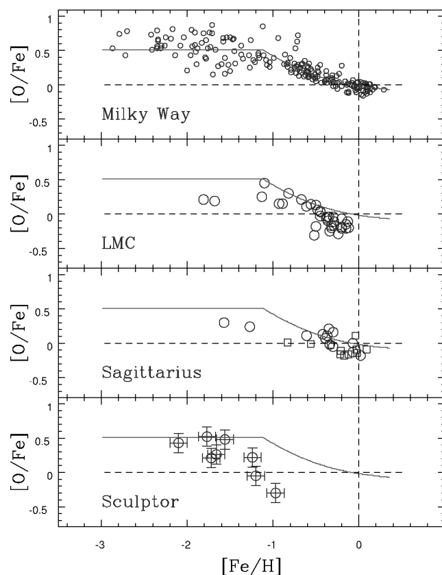
FIG. 7.— [\text{O}/\text{Fe}] vs. [\text{Fe}/\text{H}] for samples of stars in four different galaxies. The solid curve is a model fit described in the text. O abundances in the extragalactic samples are generally depleted with respect to their Galactic counterparts. [See the electronic edition of PASP for a color version of this figure.]
