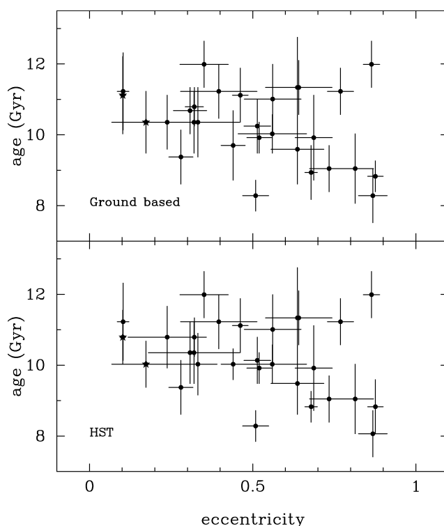
FIG. 4.—Ages for Galactic GCs from De Angeli et al. (2005) as a function of orbital eccentricity for two age data sets: ground based ( top ) and HST ( bottom ). Two metal rich clusters ( [\text{Fe}/\text{H}] > -0.8 ) are represented with star symbols.
