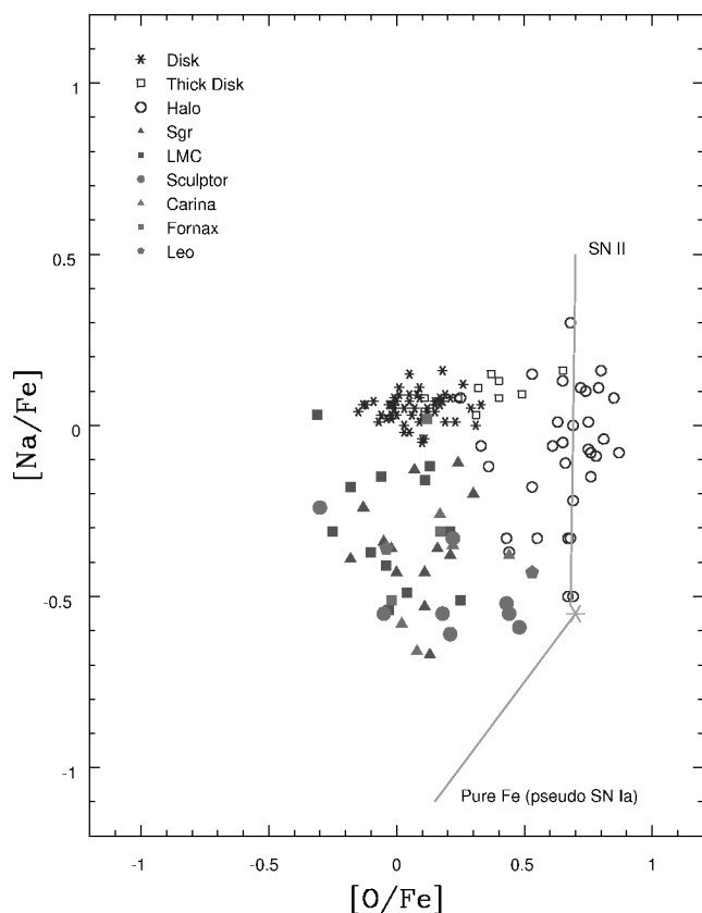
FIG. 9.—[Na/Fe] vs. [O/Fe] for stars in the Galaxy ( black symbols ) and various extragalactic samples ( gray ; see key). Solid lines represent schematic representations of contributions expected from pure SNe II and SNe Ia. [See the electronic edition of PASP for a color version of this figure.]
