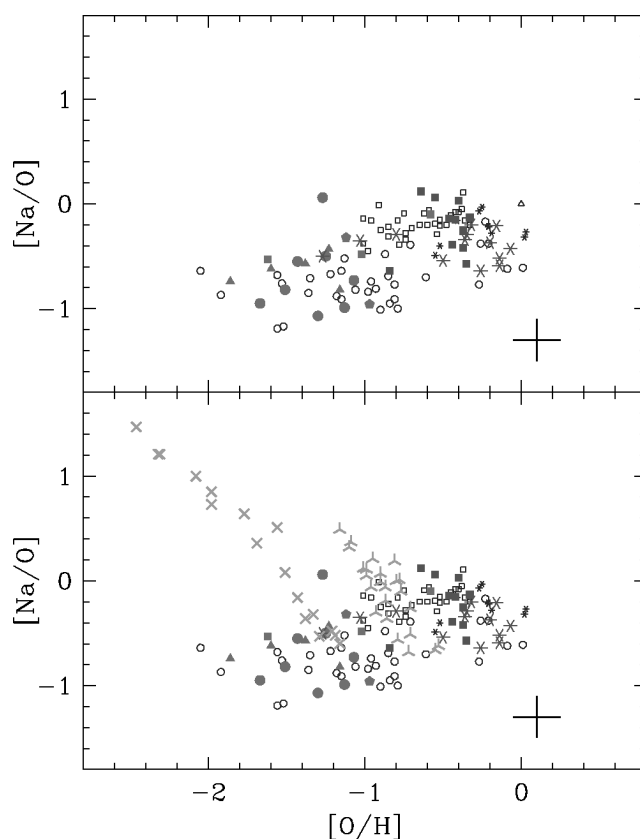
FIG. 10.—[Na/O] vs. [O/H] for ( top ) field stars in the Milky Way and dwarf galaxies (symbols as in Fig. 9) and ( bottom ) as in the top panel but also including stars from two GCs in light gray: M13 ( crosses ) and M4 ( three-pronged symbol ). [See the electronic edition of PASP for a color version of this figure.]
