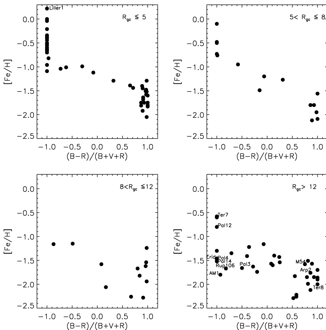
FIG. 2.—Dependence of metallicity on the color distribution of horizontal branch stars for GCs divided into four groups according to their distance from the Galactic center, following SZ78. Beyond 8 kpc there are no clusters with [Fe/H] > -1.0 except for Ter 7 and Pal 12, which are associated with the Sgr system. NGC 2419 is located in the bottom right diagram at (0.86, -2.12).
