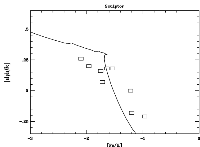
FIG. 13.— [\alpha/\text{Fe}] vs. [\text{Fe}/\text{H}] for Scl dSph giants (squares) compared to the theoretical predictions of LF04 (solid curve).
