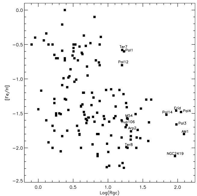
FIG. 1.—Metallicity of GCs as tabulated by Harris (2003) plotted against the log of their distances from the Galactic center in kiloparsecs. The break at 40 kpc is evident followed by six very distant GCs located at similar distances to the nearer dSph systems. Various clusters are identified.
