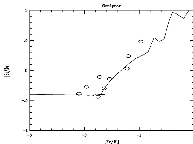
FIG. 14.— [\text{Ba}/\text{Eu}] vs. [\text{Fe}/\text{H}] for Scl dSph giants (circles) compared to the theoretical predictions of Lanfranchi et al. (2006; solid curve).
