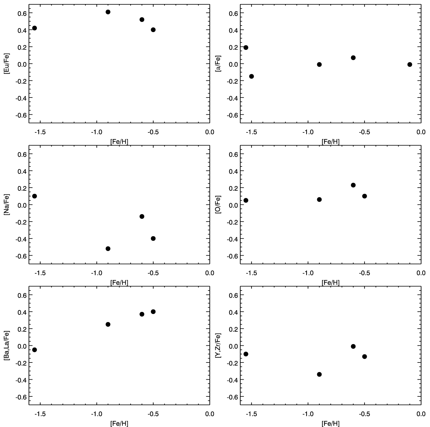
FIG. 5.—Trends of abundance of various elements or element groups with [\text{Fe}/\text{H}] in the various systems that are associated with the Sagittarius Galaxy.
