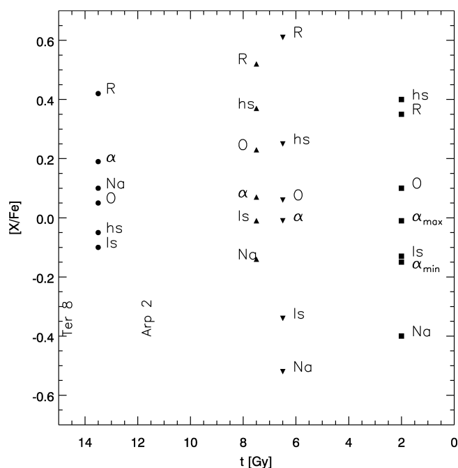
FIG. 6.—Trends of abundance of various elements or element groups with age in the various systems that are associated with the Sagittarius Galaxy.
