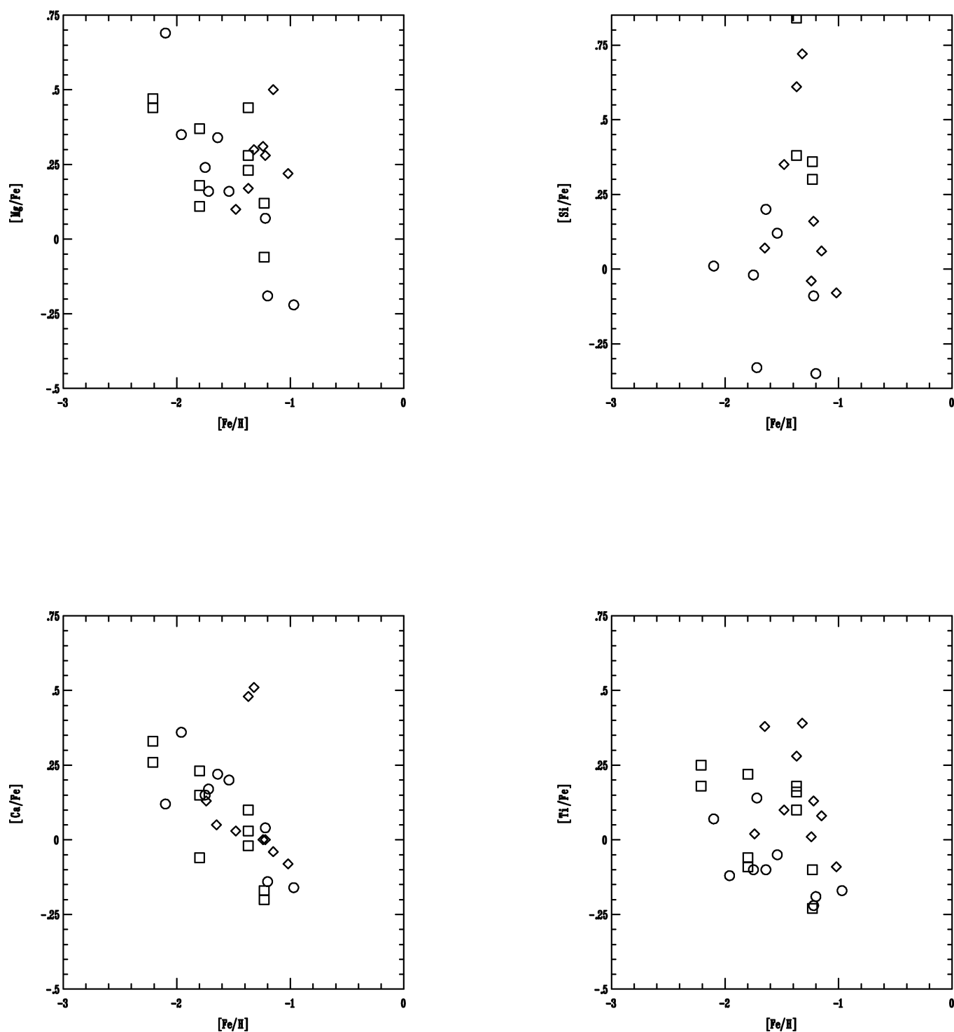
FIG. 8.—Mg, Si, Ca, and Ti abundances vs. [\text{Fe}/\text{H}] for giants in Scl ( circles ) and 2 LMC samples (J06 clusters: squares ; P07 field stars: diamonds ).
