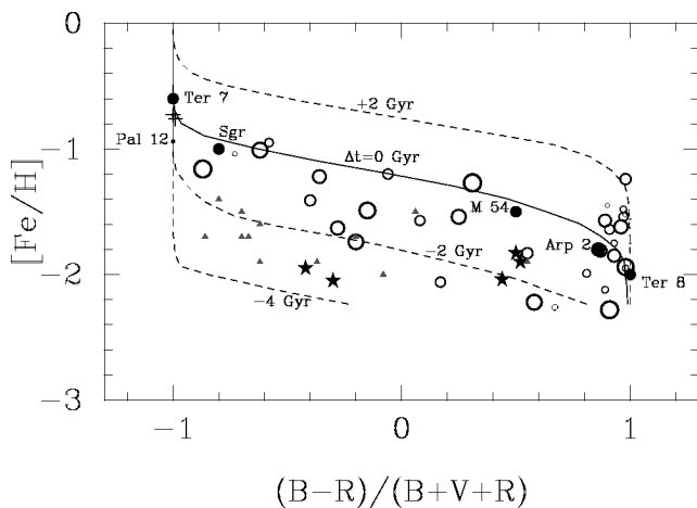
FIG. 3.—Metallicities as a function of HB type (Lee diagram) for Galactic GCs (circles), Fornax dwarf spheroidal clusters (star symbols) and mean values for dwarf spheroidals (triangles). For the Galactic GCs, the symbol size is proportional to the eccentricity. Sgr's clusters are represented with filled symbols and labeled. Equal age lines from Lee et al. (2002) are also shown. [See the electronic edition of PASP for a color version of this figure.]
