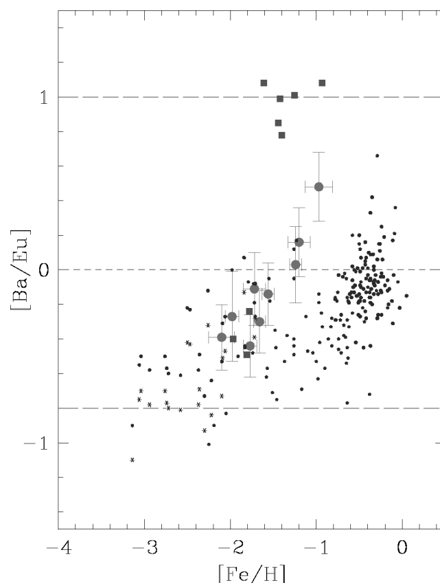
FIG. 11.—[Ba/Eu] vs. [Fe/H] for Galactic stars (same symbols as Fig. 9), dSph stars, Scl (large gray circles) and \omega Cen (dark gray squares). The dashed lines show expected abundances for pure r -process (bottom) and pure s -process (top). [See the electronic edition of PASP for a color version of this figure.]
