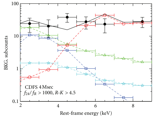
FIGURE 16: Stacked background-subtracted Chandra counts as a function of rest-frame energy, for sources with f_{24}/f_R > 1000 and R-K > 4.5 in the 4Msec CDF-S field ( filled circles ; [75]). The cyan dashed lines (stars) show the simulated spectra for the high-mass X-ray binary (HMXB) population normalized using the relation between star-formation rate and X-ray luminosity [76]. The blue dashed lines (open squares) show simulated thermal spectra corresponding to a black body with kT = 0.7\ \text{keV} . An absorbed AGN spectrum, given by a power law with \Gamma = 1.9 and a fixed N_H = 10^{24}\ \text{cm}^{-2} , is shown by the red dashed lines (open circles) . In addition, a scattered AGN component, characterized by a 1% reflection of the underlying unobscured power law, is shown by the green dashed lines (open triangles) . The resulting summed spectrum ( black solid lines ) is in very good agreement with the observed counts. The strong detection in the stacked spectrum at E > 5\ \text{keV} confirms the presence of a significant number of heavily obscured AGN in these IR-excess objects [75].
