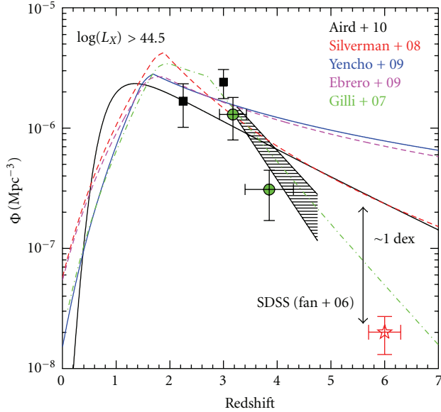
FIGURE 19: Number density of X-ray-selected AGN as a function of redshift for sources with \log l_{2-10} > 44.5 \text{ erg s}^{-1} , as published by Brusa et al. [83]. Lines show AGN luminosity functions [39, 79, 84–86] while individual measurements are shown by green circles [87] and black squares [86]. The red star at z = 6 was obtained from the optical luminosity function assuming no evolution in \alpha_{\text{ox}} . The black-shaded area shows the observations of optically bright SDSS QSOs [88].
