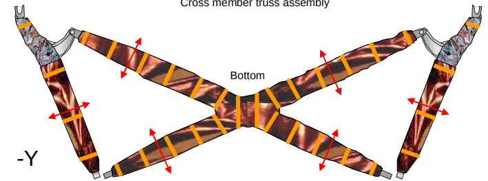
Cross member truss assembly
