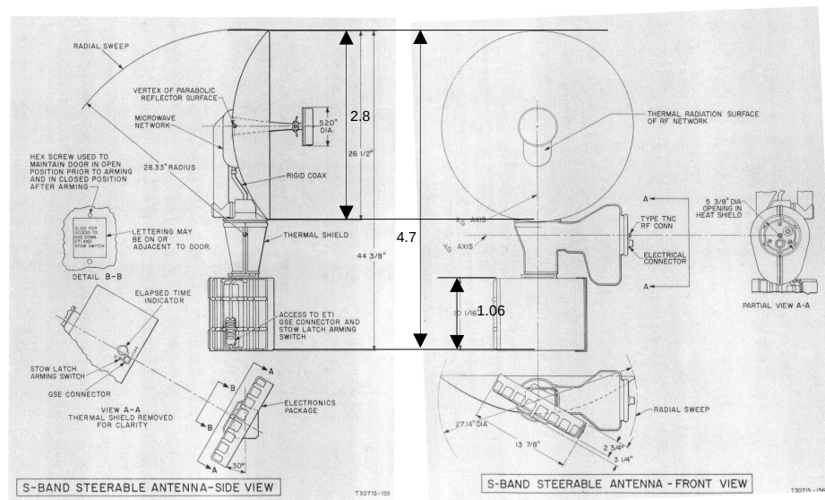
S-Band antenna
